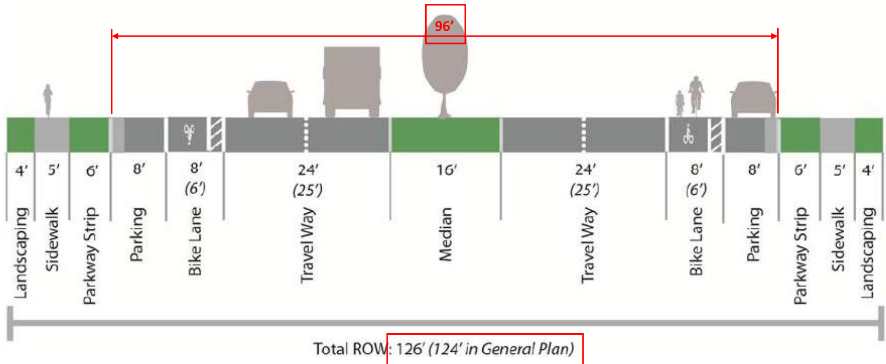
Buffered Bike Lane - Inside and Outside Buffer Options
